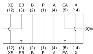
SANDWICH EXHAUST
