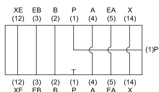
PRESSURE BLOCK
